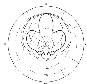
C96/30-EN - C96/30N-EN
