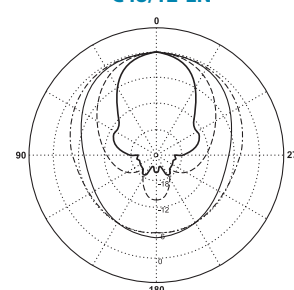
C48/12-EN
