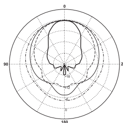
Piano verticale
